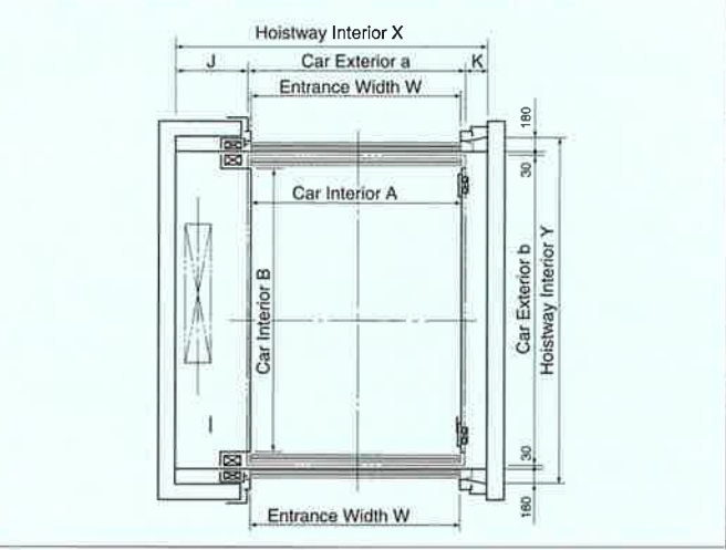
Two-panel vertical up sliding door(2500kg,3000kg)
