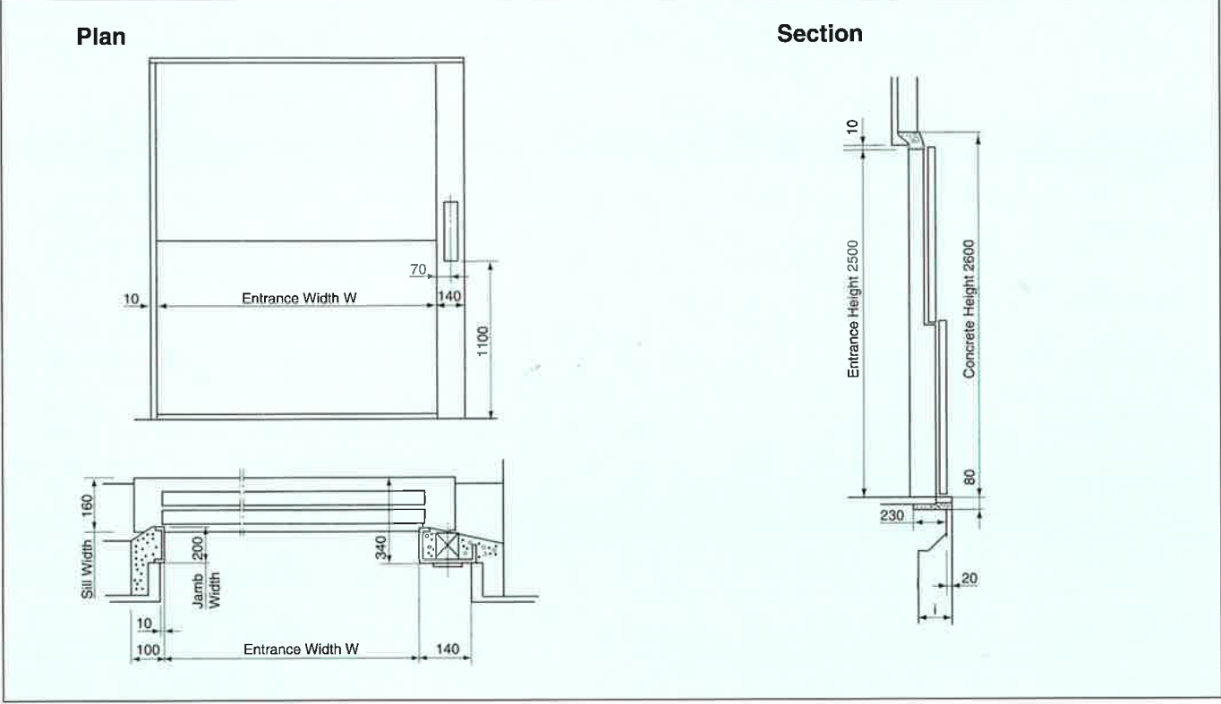
Two-panel vertical up sliding (2P-UP)
