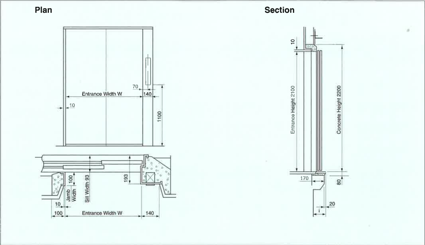
Two-panel horizontal sliding door (2S-2P)
