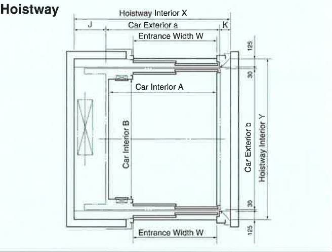
Three-panel horizontal sliding door(2500kg,3000kg)
